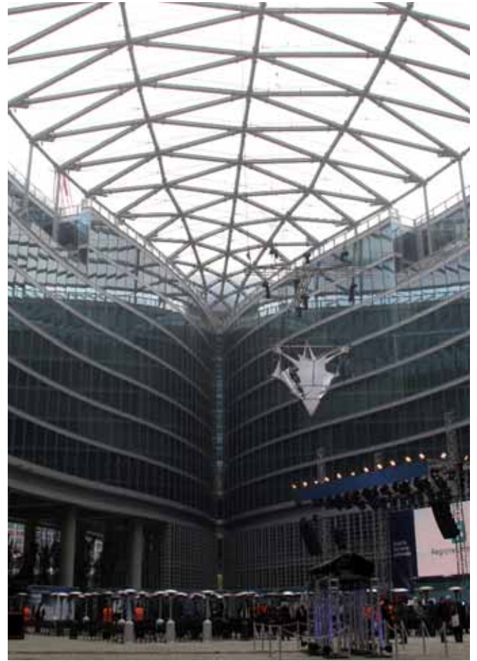
Palazzo Lombardia, Milan, Italy / Canopy roof
